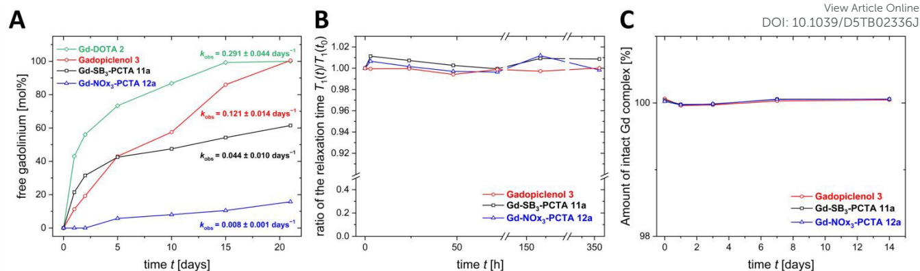
Fig. 2 (A) Released free gadolinium over time for Gd-SB 3 -PCTA 11a , Gd-NO x -PCTA 12a , gadopipiclenol 3 and Gd-DOTA 2 under acidic conditions (pH 1.2) at 37 °C, as determined by complexometric titration with arsenazo III. (B) Time-dependent relative longitudinal relaxation time T_1(t) / T_1(t_0) of gadolinium complexes (1.25 mM) in presence of ZnCl 2 (1.25 mM) in phosphate-buffered saline (PBS, pH 7.4, 37 °C), measured at 1.4 T. Measurements were performed at 0 h, 3 h, 1 day, 3 days, 7 days and 15 days. (C) Stability of Gd(III) complexes in human serum at 37 °C. Measurements were performed at 0 days, 1 day, 3 days, 7 days and 14 days.
