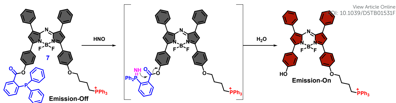
Fig. 7 Turn On mechanism of NIR mitochondrial probe 7 for HNO detection. (Redrawn the ChemDraw structures from Ref. 77)
