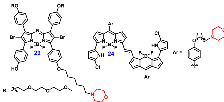
Fig. 28 Chemical structures of probes 23 and 24 . (Redrawn the ChemDraw structures from Ref. 101-102)
