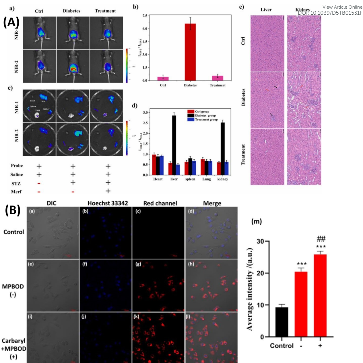
Fig. 25 (A) Confocal fluorescence imaging of diabetic mice models treated with probe 19 for visualizing endogenous HClO levels. Reproduced with permission from ref. 97, Copyright 2024 Elsevier. (B) Confocal fluorescence images of HepG2 cells stained with probe 20 under different conditions: control (probe alone), co-incubation with carboxylesterase 1 (CES1), and pre-treatment with the pesticide carbaryl followed by incubation with CES1 and the probe, illustrating CES1 activity detection and inhibition. Reproduced with permission from ref.98, Copyright 2020 Elsevier.
