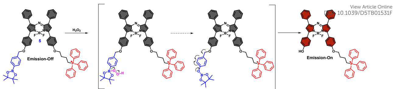
Fig. 5 Turn On mechanism of NIR mitochondrial probe 5 for \text{H}_2\text{O}_2 detection. (Redrawn the ChemDraw structures from Ref. 75)
