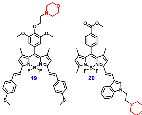
Fig. 22 Chemical structures of compounds 19 and 20 . (Redrawn the ChemDraw structures from Ref. 97-98)
