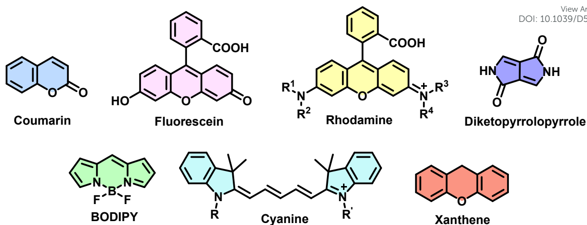
Fig. 1 Common organic fluorophores.
