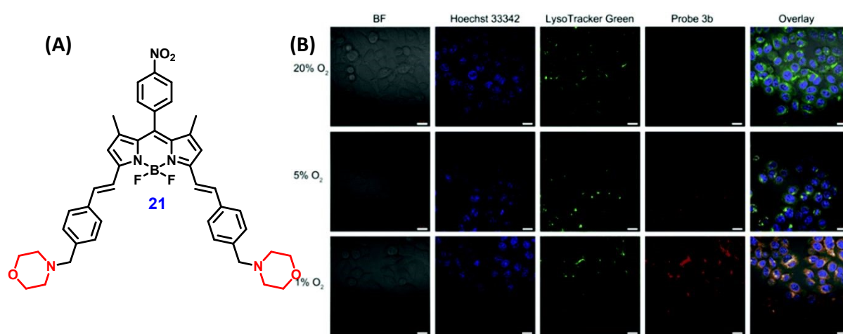
Fig. 26 (A) Chemical structure of probe 21 . (Redrawn the ChemDraw structures from Ref. 99) (B) Confocal images of HepG2 cells incubated with probe 21 under varying oxygen concentrations (hypoxic cells). Reproduced with permission from ref. 99, Copyright 2019 Royal Society of Chemistry.
