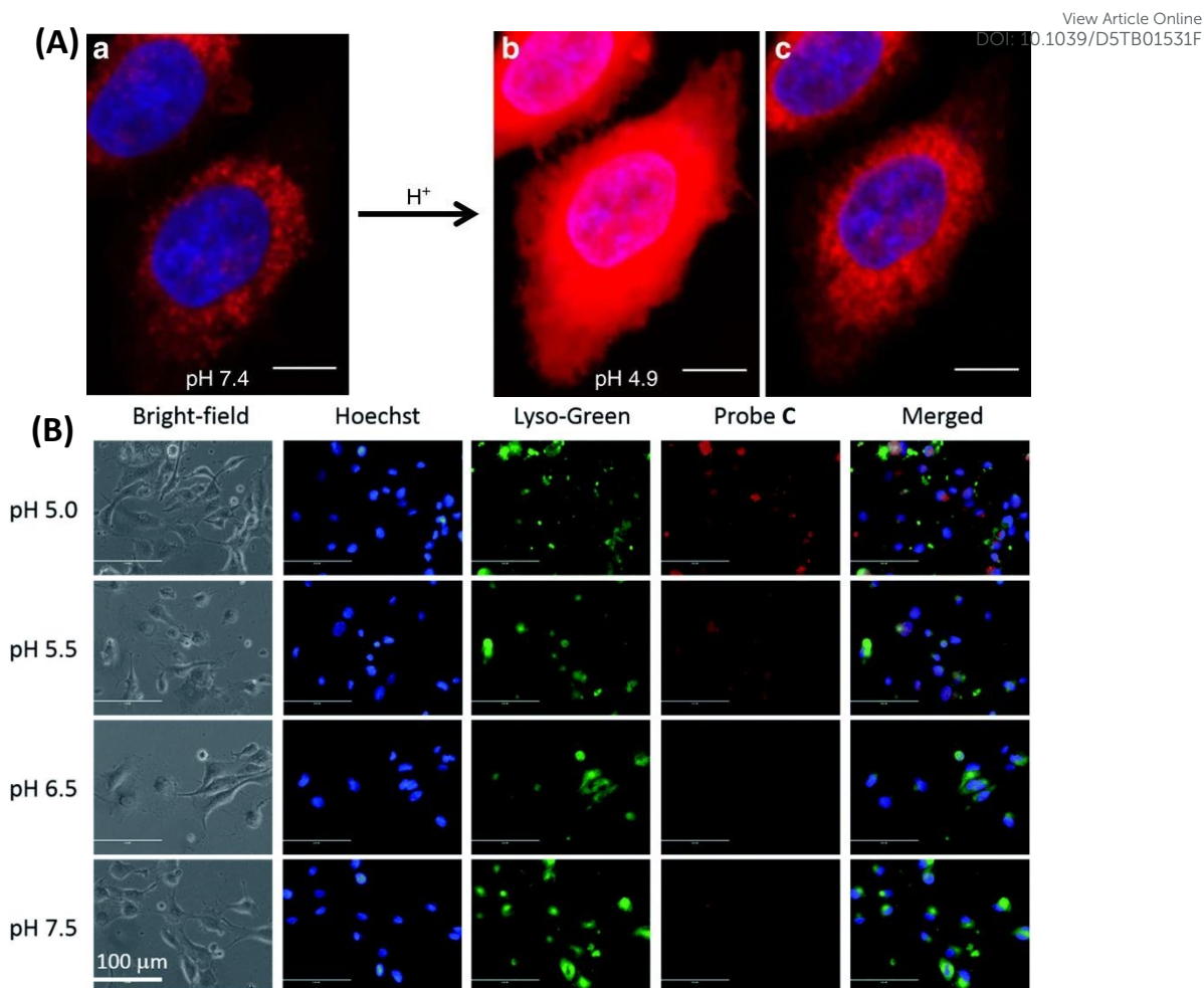
Fig. 20 (A) Confocal fluorescence images of HeLa cells incubated with probe 16 at varying pH values, demonstrating pH-responsive behavior. Reproduced with permission from ref. 94. (B) Fluorescence images of HUVEC-C cells treated with probe 17 under different pH conditions, highlighting its pH sensitivity. Reproduced with permission from ref. 95, Copyright 2015 Royal Society of Chemistry.
