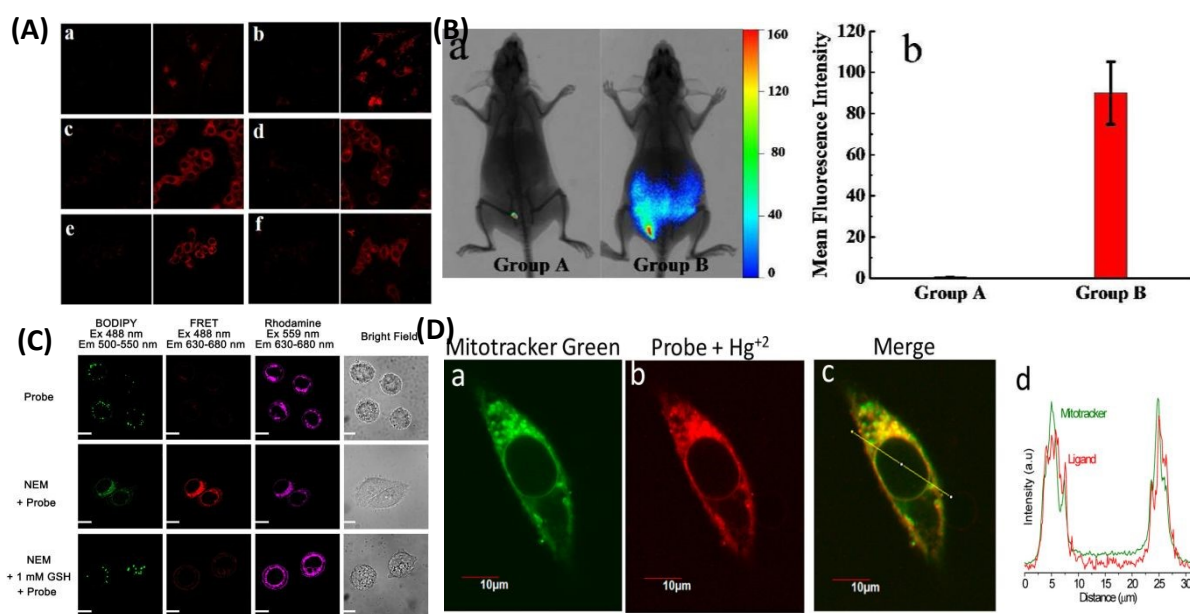
Fig. 14 (A) Fluorescence imaging of various cell lines (a-f) using probe 8 for \text{H}_2\text{S}_n detection; the left side represents control cells, while the right side shows cells treated with both probe 8 and \text{Na}_2\text{S}_2 . (B) In-vivo fluorescence images of mice models: Group A treated with probe 8 alone, and Group B with both probe 8 and \text{Na}_2\text{S}_2 ; corresponding quantitative analysis included. Reproduced with permission from ref. 78, Copyright 2015 American Chemical Society. (C) Confocal imaging of HeLa cells stained with FRET-based ratiometric probe 10 in the absence
