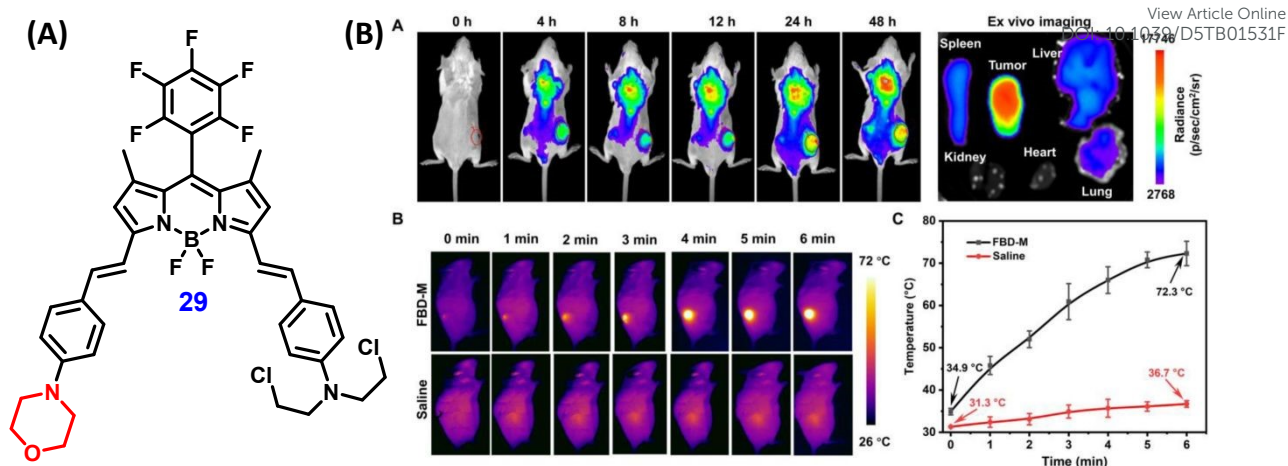
Fig. 35 (A) Chemical structure of probe 29 . (Redrawn the ChemDraw structures from Ref. 107) (B) In vivo fluorescence imaging and infrared thermography of tumors following probe 29 administration, illustrating dual-modality functionality for tumor localization and photothermal monitoring under laser irradiation. Reproduced with permission from ref. 107, Copyright 2023 Elsevier.
