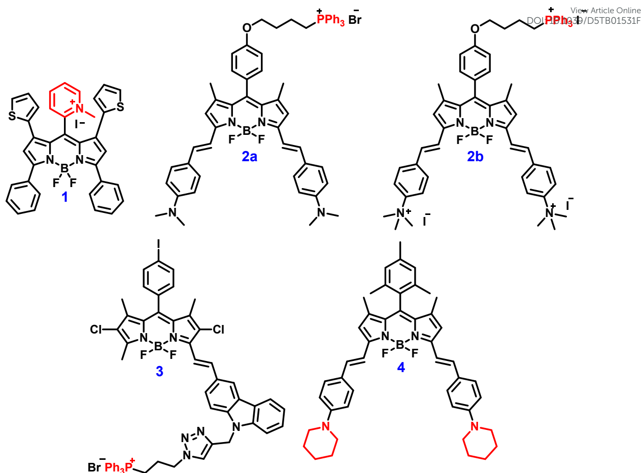
Fig. 3 Chemical structures of probes 1-4 . (Redrawn the ChemDraw structures from Ref. 71-74)
