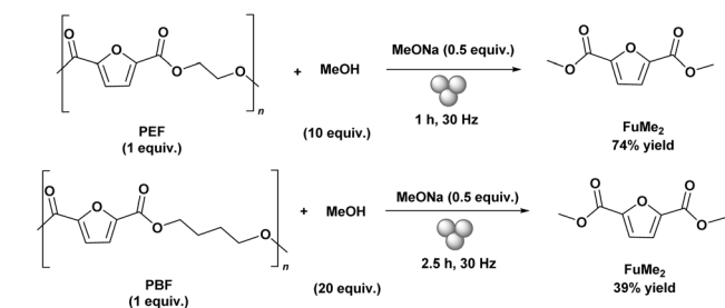
Scheme 4 Mechanochemical methanolysis of PEF and PBF (1 equiv. is based on the repeating monomer unit).
