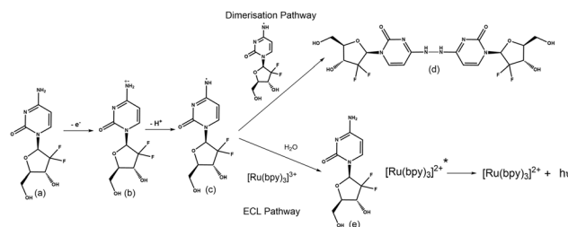
Scheme 1 Electrochemical pathway which the GEM radical can proceed down following electrocatalytic oxidation (a) and (b) at the AuNP surface, where (c) is the radical species, (d) is the dimerization product and (e) is the product of the ECL pathway alongside the required. Adapted from ref. 16.
