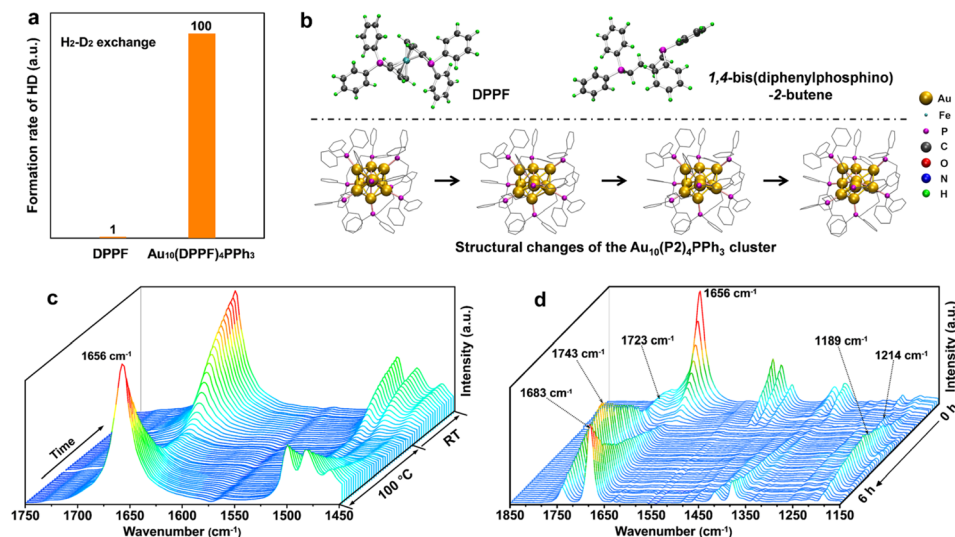
Fig. 4 (a) The normalized HD formation rate during the H 2 –D 2 exchange reaction for the Au 10 (DPPF) 4 PPh 3 cluster and the DPPF ligand, respectively. (b) Ligand substitution calculations of the Au 10 cluster. The upper panel shows the structures of the DPPF ligand (left) and the simplified P2 ligand (right). The lower panel shows the structural changes of the Au 10 (P2) 4 PPh 3 cluster during optimizations (from left to right). (c) Time-resolved in situ FTIR spectra obtained from the reaction of pyrrolidine and CO 2 performed in the high-pressure liquid cell system without the catalyst. (d) Time-resolved in situ FTIR spectra corresponding to reaction intermediate species formed in the high-pressure liquid cell during the pyrrolidine hydroformylation reaction with CO 2 and H 2 catalysed by Au 10 clusters.
