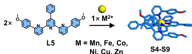
Fig. 11 Crystal structure of complexes S4–S9 assembled from ligand L5 .
