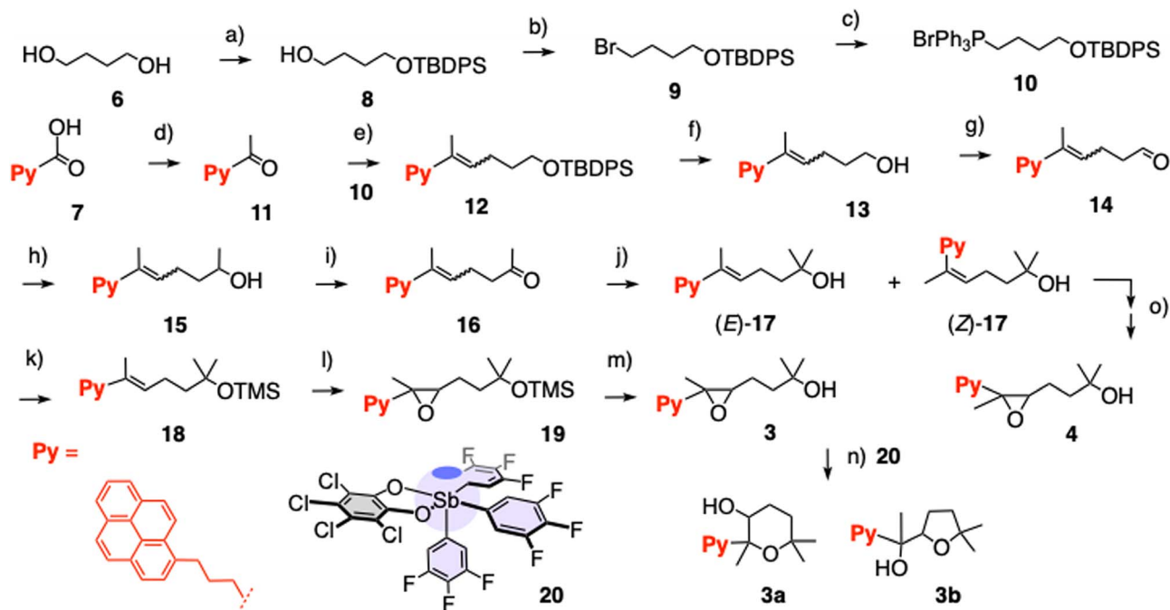
Scheme 1 Synthesis of substrate 3 and products 3a and 3b . (a) 1. NaH, THF, 0 °C, 30 min; 2. TBSPSCl, THF, 0 °C, 2 h, quant. (b) PPh 3 , CBr 4 , CH 2 Cl 2 , 0 °C to RT, 2 h, 56%. (c) PPh 3 , toluene, 150 °C, 15 h, 56%. (d) MeLi, THF, −78 °C to RT, 3 h, 70%; (e) 1. 10 , LiHDMS, THF, −78 °C to 0 °C, 30 min; 2. 11 , −78 °C to RT, 15 h, 40%. (f) TBAF, THF, 0 °C to RT, 2 h, 91%; (g) DMP, CH 2 Cl 2 , 0 °C to RT, 3 h, 61%. (h) MeMgBr, dry Et 2 O, 0 °C to RT, 1 h, quant. (i) DMP, CH 2 Cl 2 , 0 °C to RT, 3 h, 78%. (j) MeMgBr, dry Et 2 O, 0 °C to RT, 1 h, 83% ( E + Z ). (k) DMAP, Et 3 N, TMSCl, CH 2 Cl 2 , RT, 1 h, 82%. (l) m -CPBA, CH 2 Cl 2 , 0 °C to RT, 1 h, 83%. (m) TBAF, THF, 0 °C to RT, 2 h, 94%. (n) 20 , CH 2 Cl 2 , RT, 30 min, 95% (81% 3a , 14% 3b ). (o) See ESI.†
