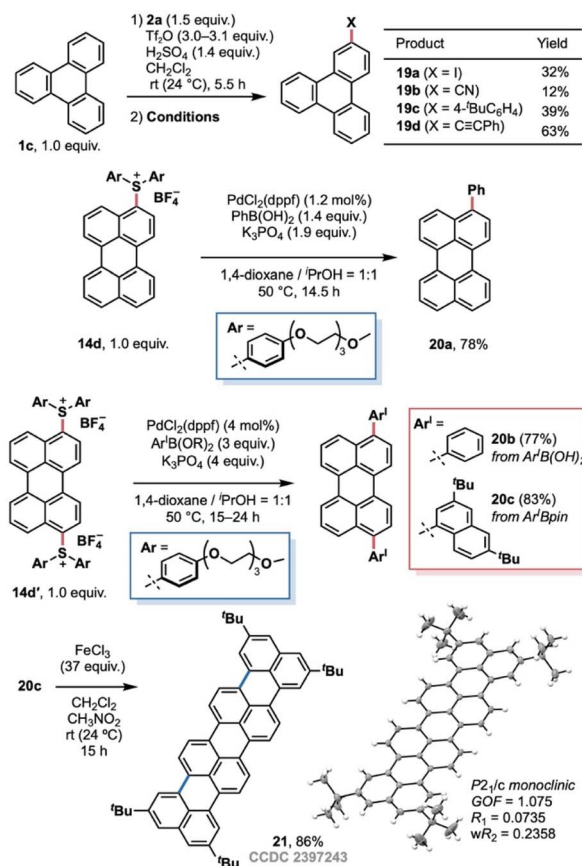
Scheme 3 Transformation of PAH-sulfonium salts. Conditions for the synthesis of 19a : \text{RuCl}_2(\text{bpy})_3 \cdot 6\text{H}_2\text{O} (3.3 mol%), \text{CuBF}_4(\text{MeCN})_4 (1.0 equiv.), Lil (9.8 equiv.), MeCN/DMSO, blue LED, rt (23 °C), 21 h; conditions for the synthesis of 19b : \text{RuCl}_2(\text{bpy})_3 \cdot 6\text{H}_2\text{O} (2.5 mol%), \text{CuBF}_4(\text{MeCN})_4 (1.3 equiv.), \text{N}^t\text{Bu}_4\text{CN} (2.5 equiv.), MeCN, blue LED, rt (24 °C), 21 h; conditions for the synthesis of 19c : \text{PdCl}_2(\text{dppf}) (2.2 mol%), (4- tert -butylphenyl)boronic acid (1.4 equiv.), \text{K}_3\text{PO}_4 (2.0 equiv.), EtOH/1,4-dioxane, 50 °C, 48 h; conditions for the synthesis of 19d : \text{PdCl}_2(\text{dppf}) (2.7 mol%), phenylacetylene (1.4 equiv.), Cul (21 mol%), N -methylmorpholine (2.1 equiv.), 1,4-dioxane, 40 °C, 48 h.
