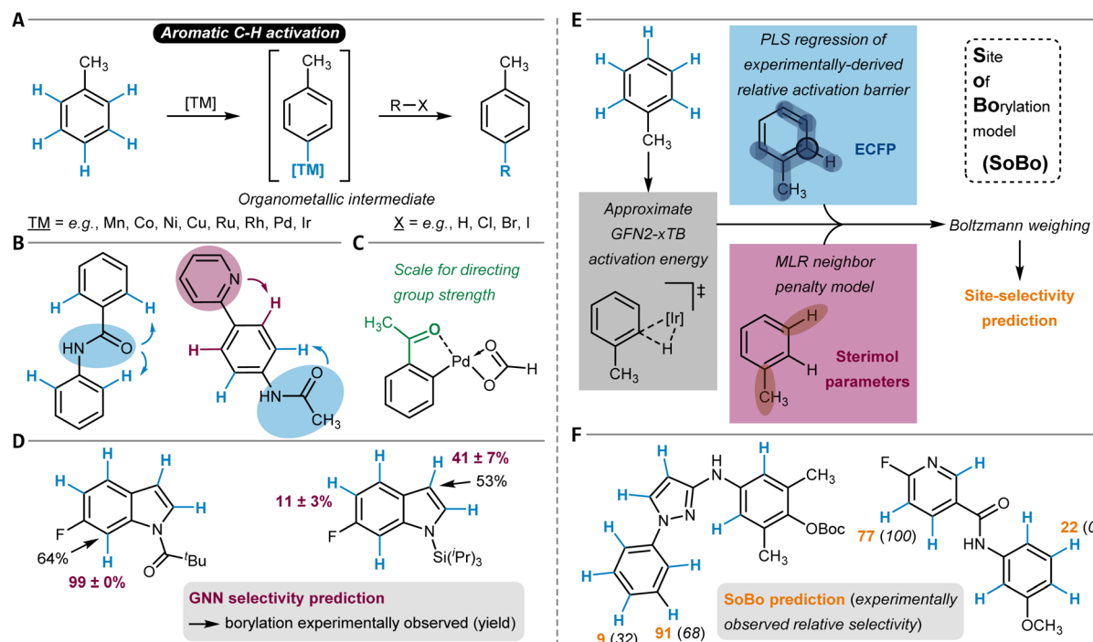
Fig. 9 (A) Schematic reaction mechanism of a C-H activation-mediated C aryl -H substitution reaction. (B) A single directing group favoring two different sites (left) and two different directing groups favoring two different sites (right) during C-H activation. (C) Example of the palladacycle intermediate used by Tomberg et al. to computationally construct a scale for directing group strength. The example directing group is highlighted in green. (D) Borylation site-selectivity predictions made by a three-dimensional GNN model and comparison to the experimental observations. The predicted percentages and respective standard deviations were obtained by applying the model to ten different conformers of the substrate molecule. (E) Schematic representation of the Site of Borylation (SoBo) model architecture and (F) two of its prediction examples in comparison to the experimental observations.
