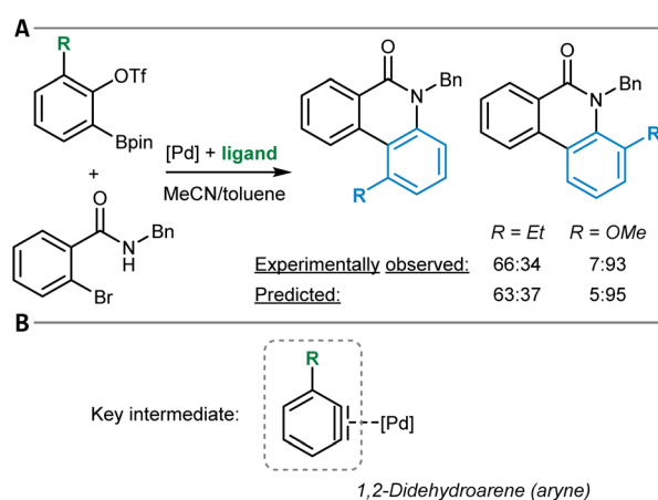
Fig. 18 (A) Palladium-catalyzed annulation of ortho -borylaryl triflates and the two possible reaction products with experimentally observed regioselectivities and the respective predictions from a linear model. The Hammett and Charton parameters of the R substituent and the cone angle of the applied ligand at palladium were used to predict regioselectivity. (B) The key intermediate of the reaction shown in (A), which is the palladium complex of the in situ -generated aryne.
