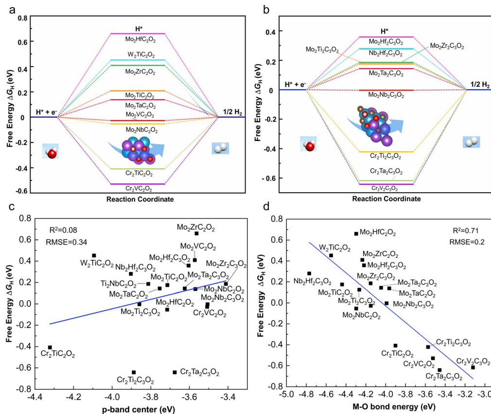
Fig. 5 (a and b) HER free energy diagrams of M'_2M''C_2O_2 and M'_2M''C_3O_2 under standard conditions, respectively. (c and d) Relationships between \Delta G_{H^+} and descriptors including (c) the p-band center of the oxygen functional group and (d) the bond energy between the first-layer transition metal and oxygen of different MXene systems, respectively.
