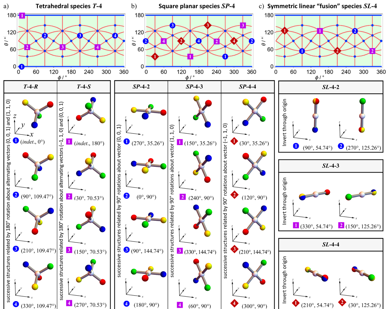
Fig. 5 Locations ( \phi , \theta ) and orientation permutations of (a) tetrahedral T-4 , (b) square planar SP-4 , and (c) symmetric linear SL-4 "fusion" species in the AB_4 T-4 E-mode configuration space. Locations are shown on the equirectangular projection of the configuration space (upper panels). For the depictions of the species, offset axes are shown for orientation purposes only. Colours differentiate B-atoms and do not denote specific elements.
