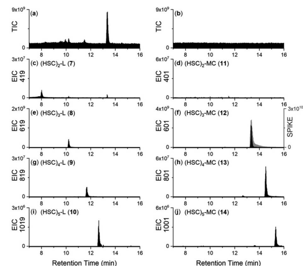
Fig. 3 LC-MS traces from solutions of 2 with MgCl_2 and ATP, incubated ( 37^\circ C , 2 h, pH 8) in the presence (a) or absence (b) of StDesD , as detected by TIC (a and b), or shown as an EIC with values set to report the [M + H]^+ adducts of (c) 7 , (d) 11 , (e) 8 , (f) 12 , (g) 9 , (h) 13 , (i) 10 , or (j) 14 . The trace in gray (f) was acquired from the solution following the addition of authentic 12 .
