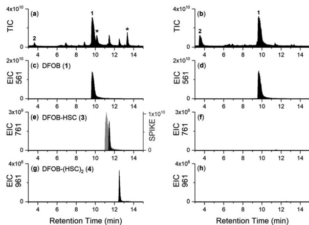
Fig. 1 LC-MS traces from solutions of 1 and 2 with MgCl_2 and ATP, incubated ( 37^\circ C , 2 h, pH 8) in the presence (a, c, e and g) or absence (b, d, f and h) of StDesD , as detected by TIC (a and b), or shown as an EIC with values set to report the [M + H]^+ adducts of (c and d) 1 , (e and f) 3 , or (g and h) 4 . The trace in gray (e) was acquired from the solution following the addition of authentic 3 . Asterisk signals in (a) are due to species assembled from 2 alone.
