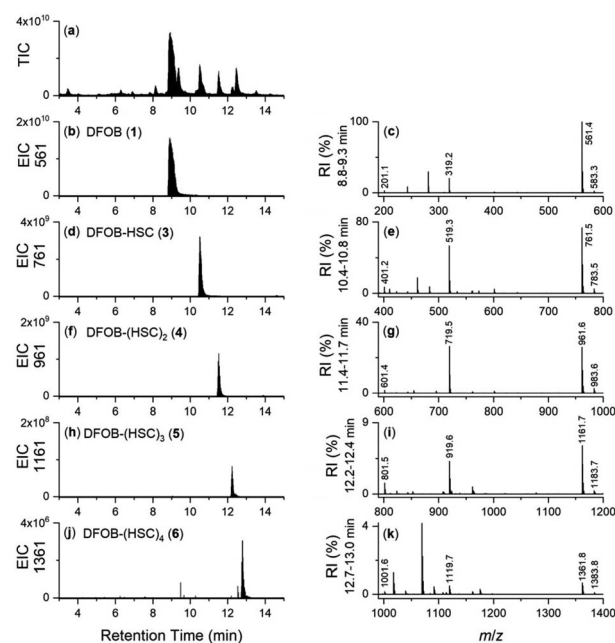
Fig. 2 LC-MS traces from solutions of 1 and 2 with MgCl_2 and ATP, incubated ( 37^\circ C , 2 h, pH 8) in the presence of StDesD , as detected by TIC (a), or shown as an EIC with values set to report the [M + H]^+ adducts of (b) 1 , (d) 3 , (f) 4 , (h) 5 , or (j) 6 , with signature regions of the MS fragmentation pattern aligned at right (c, e, g, i and k).
