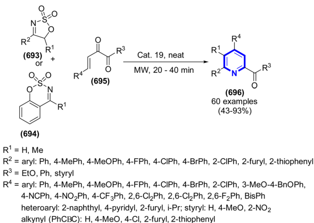
Scheme 194 Synthesis of pyridines catalyzed by Cat. 19.
