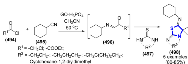
Scheme 132 Synthesis of hydroxy-thiazolidine-4-carboxylate derivatives catalyzed by phosphoric acid supported on graphene oxide.
