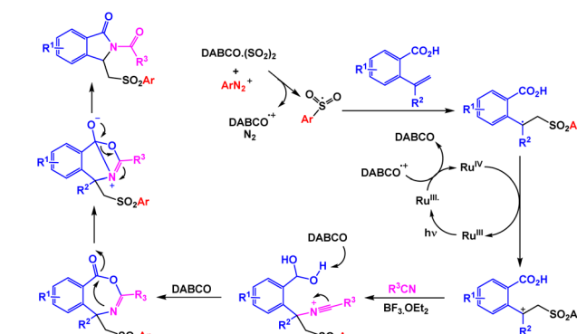
Scheme 26 Rational mechanism for synthesis of sulfonated 1-isoindolinones via ruthenium-catalyzed one-pot four-component reaction of 2-vinylbenzoic acids, aryldiazonium tetrafluoroborates, the sulfur dioxide surrogate DABCO- (\text{SO}_2)_2 , and nitriles.
