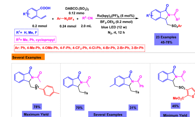
Scheme 25 Synthesis of sulfonated 1-isoindolinones via ruthenium-catalyzed one-pot four-component reaction of 2-vinylbenzoic acids, aryldiazonium tetrafluoroborates, the sulfur dioxide surrogate DABCO- (\text{SO}_2)_2 , and nitriles.
