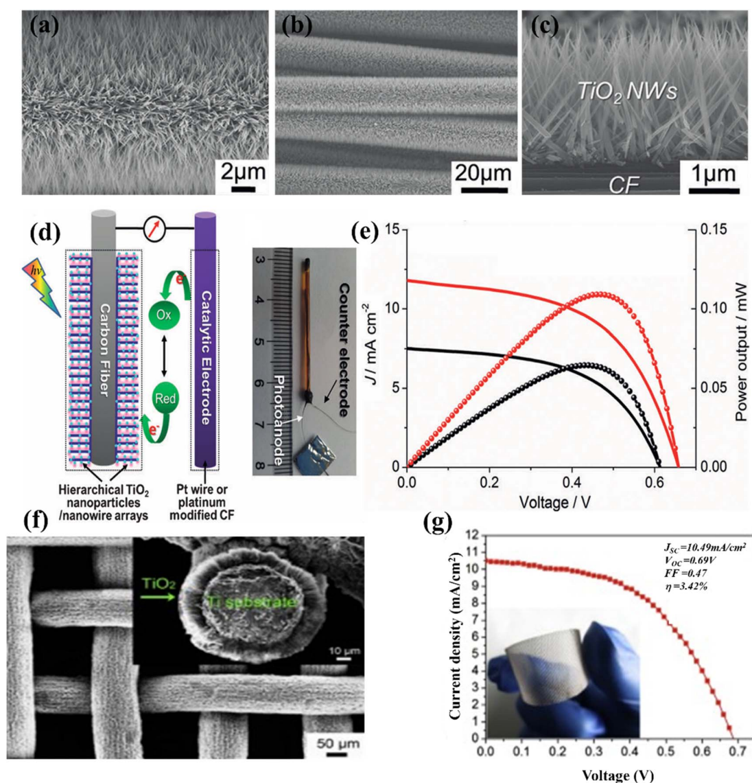
Fig. 10 (a–c) FESEM images of hierarchical TiO 2 nanowire arrays grown over the CF substrate at 190 °C for 80 minutes, (d and e) schematic of wire DSSC consisting TiO 2 nanoparticle and nanowires and Pt-modified CF counter electrodes and consequent J – V analysis, (f and g) low-magnification FESEM images of the TiO 2 NWAs on Ti mesh substrates and respective J – V performance. 72
