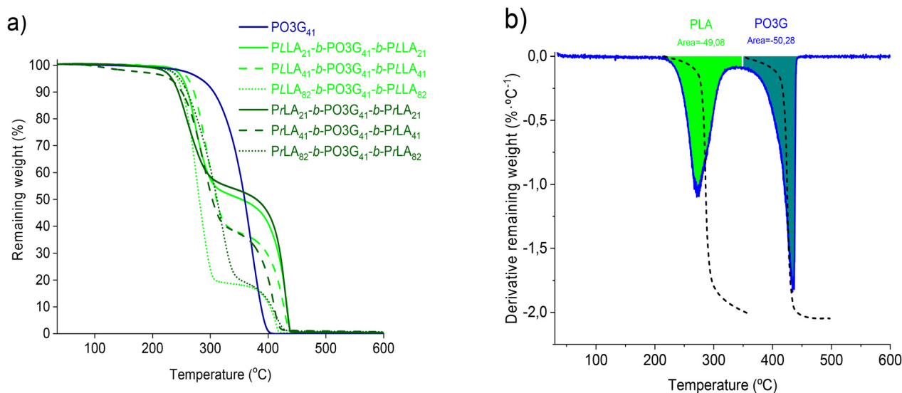
Fig. 5 (a) TGA traces of the PO3G 41 and PLA m -b-PO3G 41 -b-PLLA m copolymers and (b) the derivative curve of the PLLA 21 -b-PO3G 41 -b-PLLA 21 copolymer.
