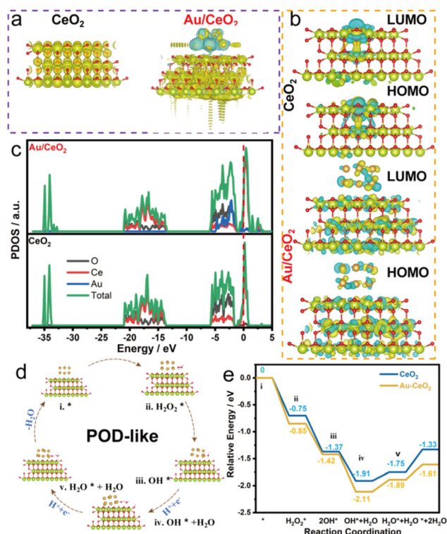
Fig. 5 (a) Charge density difference illustration of \text{CeO}_2 and \text{Au/CeO}_2 . (b) HOMO–LUMO energy levels and the interfacial diagrams of the molecular orbitals for \text{CeO}_2 and \text{Au/CeO}_2 . (c) Density of states of \text{CeO}_2 and \text{Au/CeO}_2 . (d) Proposed reaction pathways of the POD-like reaction. (e) Corresponding free energy diagrams of \text{CeO}_2 and \text{Au/CeO}_2 for the POD-like reaction.
