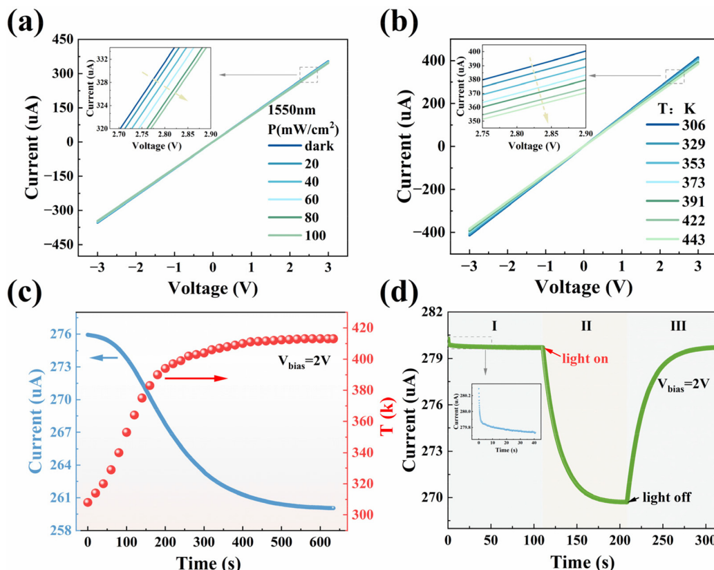
Fig. 5 Negative photoresponse characteristics of \text{Bi}_2\text{Se}_3 - \text{PtSe}_2 heterojunction photodetectors and the whole process of their photocurrent generation. I–V characteristic curves for different optical power densities (a) and different temperatures under 1550 nm illumination (b). The current generated by the device gradually decreased when the light intensity increased, and the resistance increased accordingly. At the same time, with the increase in temperature, the trend for the device current was the same as that for the increase in light intensity. (c) Curves of the current of the device as a function of temperature in the absence of light. The curves show that the temperature change caused a change in the current of the device and the current tended to decrease as the temperature increased. (d) The entire process of photocurrent generation, V_{\text{bias}} = 2\text{V} .
