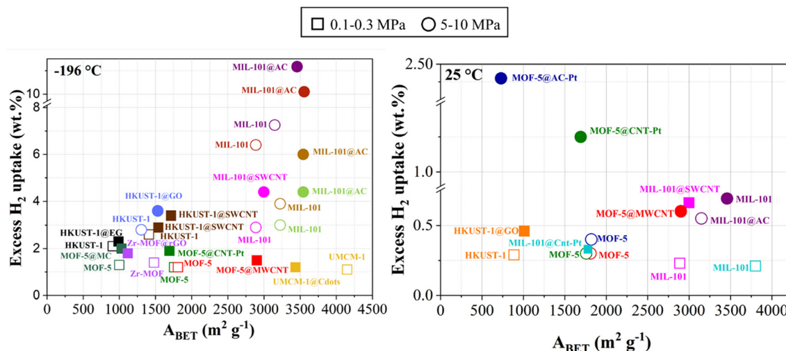
Fig. 9 Excess H 2 uptake of MOF hybrids reported in recent studies at −196 °C (left) and 25 °C (right) (○● ref. 220); (□■ ref. 221); (□■ ref. 222); (□■ ref. 223); (○●, □■ ref. 131); (□■, ○● ref. 207); (□■ ref. 175); (○● ref. 224); (□■ ref. 214); (○●, □■ ref. 158); (○●, □■ ref. 218); (○●, □■ ref. 159); (○● ref. 204); (□■ ref. 225).
