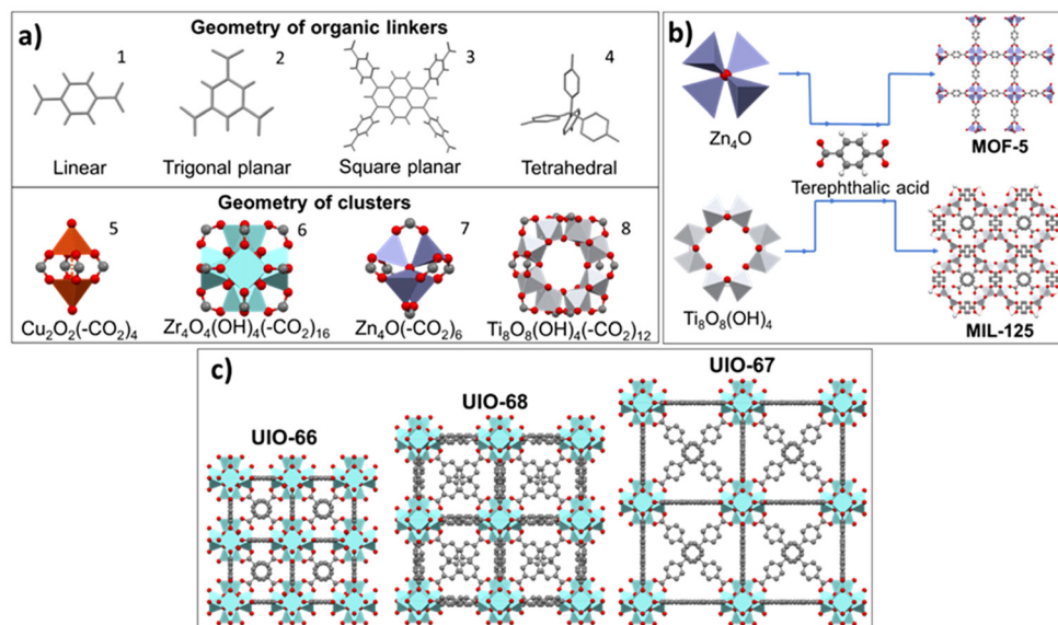
Fig. 1 (a) Geometry of some organic linkers (1: BDC; 2: BTC; 3: H4TBAPY and 4: tetraphenylmethane) (adapted from ref. 12 and 13), and geometry of some clusters; (b) assembly of two different clusters with the same organic linker to obtain two MOFs; (c) assembly of the same cluster ( \text{Zr}_4\text{O}_4(\text{OH})_4(-\text{CO}_2)_{16} ) with 3 linkers to obtain three different MOFs.
