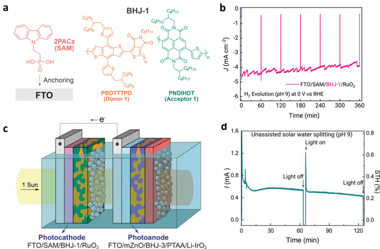
Fig. 19 (a) Molecular structures of 2PACz, PBDTTTPD, and PNDIHDT. (b) CA curves at 0 V_{\text{RHE}} of the FTO/2PACz(SAM)/BHJ-1 (PBDTTTPD:PNDIHDT)/ \text{RuO}_2 photocathode in 0.1 M NaBi buffer adjusted to pH 9. (c) Schematic illustration of the OS-based PEC tandem cell with the FTO/SAM/BHJ-1/ \text{RuO}_2 photocathode and the FTO/mZnO/BHJ-3 (PBDTTTPD:PNDITCVT)/PTAA/Li-IrO 2 photoanode for overall solar water splitting. (d) Photocurrent without an applied potential and STH efficiency of the OS-based PEC tandem cell in 0.1 M NaBi buffer adjusted to pH 9 under 1 sun illumination. Adapted with permission. 32 Copyright 2022, Wiley-VCH GmbH.
