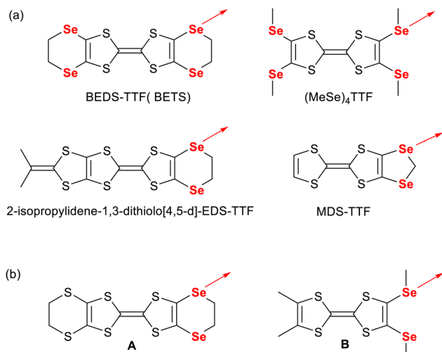
Scheme 1 Reported selenated TTFs engaged in ChB interactions in their salts. The red arrow shows the direction of the expected ChB interaction toward Lewis bases upon the activation of TTF through oxidation.
