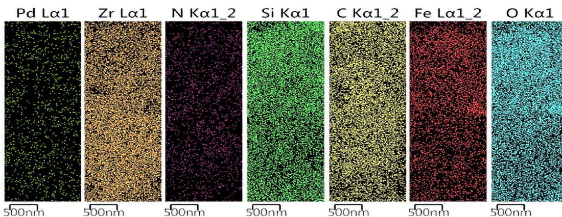
Fig. 5 EDX-mapping of \text{Fe}_3\text{O}_4@\text{MCM-41}@UiO-66/\text{SB-Pd} .
