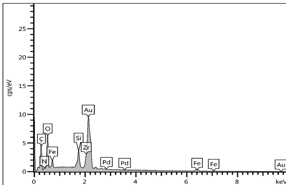
Fig. 4 EDX spectrum of \text{Fe}_3\text{O}_4@\text{MCM-41}@UiO-66/\text{SB-Pd} .
