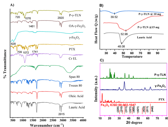
Fig. 3 FTIR analysis of all individual components and TLN loaded with PTX and \gamma -Fe _2 O _3 (A). Melting point profile of lauric acid and loaded nanocarriers (B) and XRD pattern identifying the significant 2\theta values of PTX, \gamma -Fe _2 O _3 , and P- \gamma -TLN (C).
