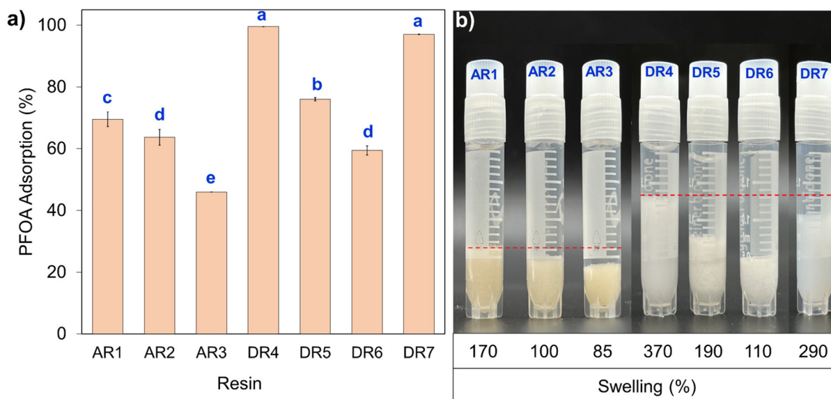
Fig. 4 (a) The efficiency of APTEMAC and DADMAL resins for the adsorption of PFOA from water. Different letters indicate significantly different values between groups as analyzed by one-way ANOVA with Tukey post-hoc test ( p < 0.050 ). (b) The visual observation of the swelling of APTEMAC and DADMAL resins in water. Red dashed lines indicate top of the highest swelled resin levels for comparison.
