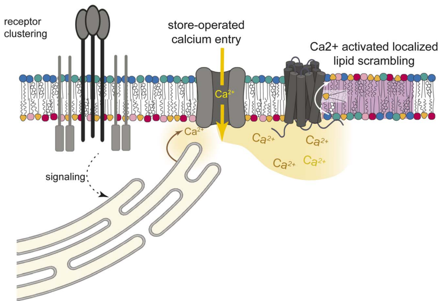
Fig. 5 Schematic of hypothesized cellular mechanism of lipid scrambling downstream of immune activation. Engagement of immune receptors activates calcium mobilization through IP 3 and SOCE. The resulting increase in intracellular calcium activates PM resident scramblases to locally release lipid asymmetry.
