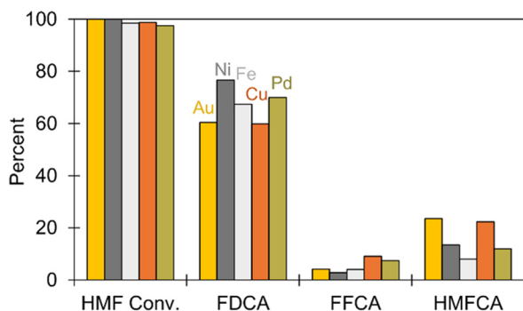
Fig. 6 Yields and conversion of adding metals to an Au/MgAlO x catalyst. Reaction conditions: 70:1 HMF:metal molar ratio, 0.25 wt% initial HMF, T = 363\text{ K} , P_{\text{O}_2} = 0.5\text{ MPa} , and t = 2\text{ h} . 73
