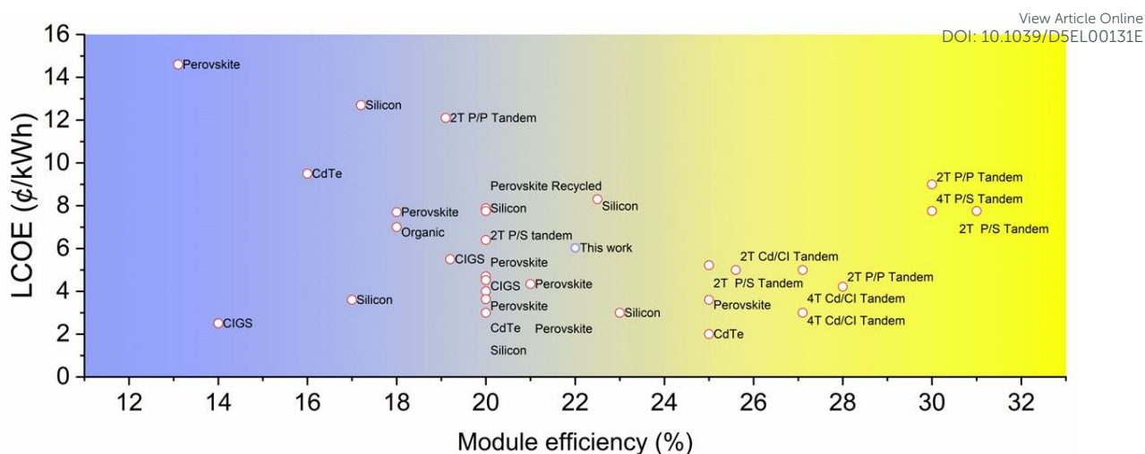
Fig. 7 LCOE vs. module efficiency comparison across various PV technologies published in the literature, with LCOE data collected from references 84–104 .
