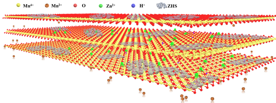
Fig. 1 With conflicting electrochemical reaction mechanisms in aqueous Zn–MnO 2 batteries, possible proposed storage mechanisms include Mn electrodisso- lution–deposition, H + and/or Zn 2+ intercalation–deintercalation and ZHS (Zn 4 (OH) 6 SO 4 ·nH 2 O) deposition–dissolution are depicted in δ-MnO 2 , a layered phase, from a pool of available MnO 2 polymorphs.
