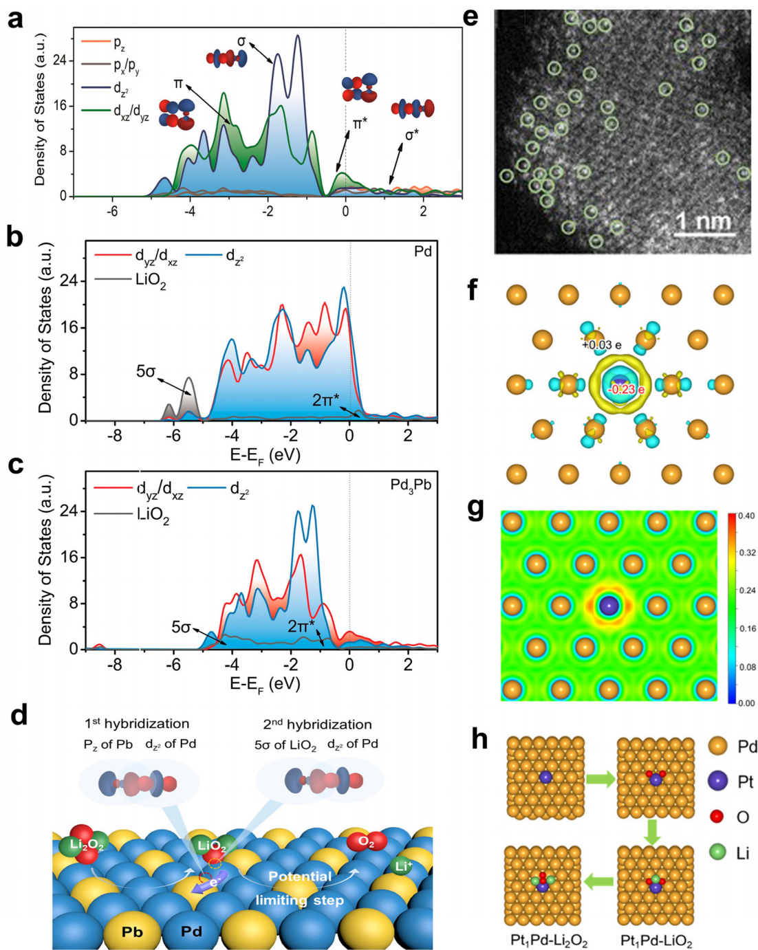
Fig. 13 (a) DOS of Pd d_{zz} , d_{xz/yz} orbitals and Pb p_x , p_y , p_z orbitals after intra-molecular p-d orbital hybridization in Pd 3 Pb. (b) DOS of Pd 4d d_{yz}/d_{xz} and d_{z^2} orbitals in Pd. (c) DOS of Pd 4d d_{yz}/d_{xz} and d_{z^2} orbitals in Pd 3 Pb with adsorbed LiO 2 . (d) Schematic representation of cascade orbital-oriented hybridization from intra-molecular Pb-Pd p-d hybridization in Pd 3 Pb to inter-molecular orbital hybridization between Pd 3 Pb (Pd 4d_{xz/yz} and 4d_{z^2} ) and LiO 2 ( 2\pi^* and 5\sigma ), using the d_{z^2} orbital along the z-axis as an example. 115 (e) AC-HAADF-STEM image of the Pt 1 Pd alloy (single-atom Pt marked with green circles). (f) ELF values of Pt 1 Pd. (g) Charge density difference distribution (regions of electron enrichment and depletion) in Pt 1 Pd. (h) Schematic representation of the discharge pathway of a Li-O 2 battery on the Pt 1 Pd surface. 40
