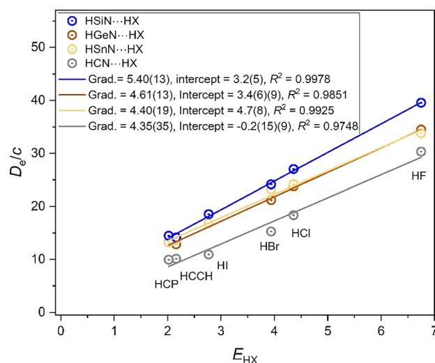
Fig. 8 Graphs of D_e/c versus E_{HX} for the four series HMN...HX ( M = C, Si, Ge, Sn , ( X = F, Cl, Br, I, CCH, CP ) in which the atom M adjacent to that directly involved in the hydrogen bond belongs to Group 14.
