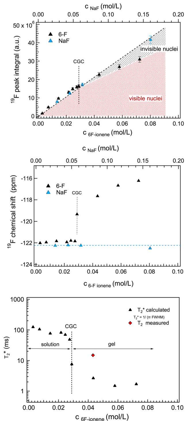
Fig. 7 (top) Integrated intensities of NMR peaks for ^{19}\text{F} nuclei as a function of 6-F concentration in \text{D}_2\text{O} . CGC is marked by a black dashed vertical line. (center) Position of the singlet obtained in ^{19}\text{F} NMR spectra of the ionene series and a reference NaF series, for which a narrow sharp singlet is observed at all concentrations. Error bars are smaller than the symbol size. (bottom) T_2^* relaxation time as a function of 6-F concentration, calculated from FWHM of the ^{19}\text{F} singlet. The red diamond marker presents the “true” T_2 value obtained using Carr–Purcell sequence with Gill–Meiboom modification. Error bars represented by the symbol size.
