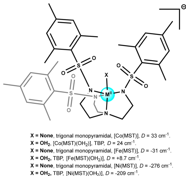
Fig. 17 Schematic representation of complexes 19 and 19' (left); CASSCF-computed principal magnetic anisotropy axes ( D_{xx} , D_{yy} , and D_{zz} ) are shown as pink dotted lines for the cobalt complex (a, 19a and b, 19a' ). The blue arrow highlights the direction and orientation of the D_{zz} , while the green arrows represent the molecular orientation axes (right), 94 adapted/reproduced from ref. 94 with permission from The Royal Society of Chemistry, 94 copyright 2018.
