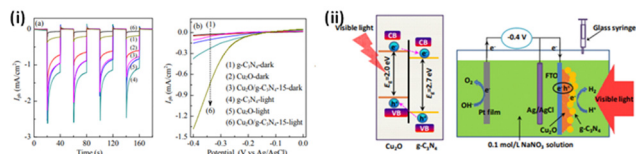
Fig. 8 (i) Transient photocurrent response at a bias potential of -0.4 \text{ V} (vs. Ag/AgCl) under visible light: [(1) \text{Cu}_2\text{O} ; (2) \text{Cu}_2\text{O}/\text{g-C}_3\text{N}_4-5 ; (3) \text{Cu}_2\text{O}/\text{g-C}_3\text{N}_4-10 ; (4) \text{Cu}_2\text{O}/\text{g-C}_3\text{N}_4-15 ; (5) \text{Cu}_2\text{O}/\text{g-C}_3\text{N}_4-20 ; (6) \text{g-C}_3\text{N}_4 ]. (b) Linear sweep voltammograms of \text{Cu}_2\text{O} , \text{g-C}_3\text{N}_4 and \text{Cu}_2\text{O}/\text{g-C}_3\text{N}_4-15 films in the dark and under visible light. (ii) Schematic pathway for photoelectron transfer and the photoelectrochemical process in \text{Cu}_2\text{O}/\text{g-C}_3\text{N}_4 film under visible light irradiation. Reprinted from ref. 151 with permission.
