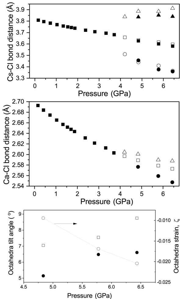
Fig. 9 Top: Variation in Cs–Cl bonds within the CsCl_n polyhedra of CsCaCl_3 with increasing pressure. Filled squares represent the the cubic phase. Unfilled circles, squares and triangles the tetragonal phases and the filled circles, squares and triangles the rhombohedral. Middle: Variation in the Ca–Cl bonds in the CaCl_6 octahedra with pressure. Filled squares in the cubic phase, unfilled triangles the tetragonal phase and the filled circles in the rhombohedral phase. Bottom: Shows the variation in the octahedra tilts in the tetragonal ( \phi ) and rhombohedral ( \omega ) phases with pressure and the variation in octahedra strain ( \zeta ) in the rhombohedral phase (unfilled circles) as defined in the main text.
