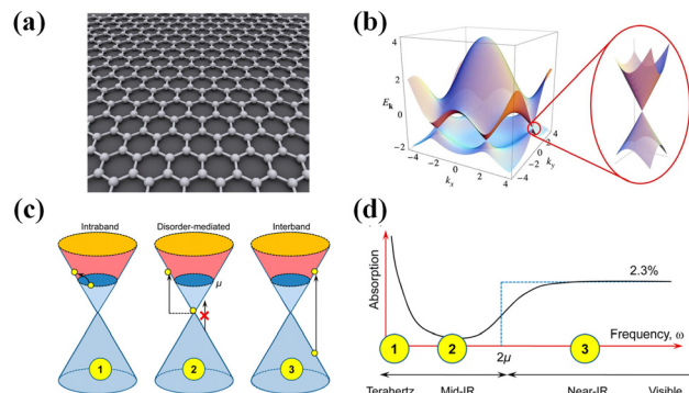
Fig. 2 2D material graphene. (a) Crystal structure of graphene. 65 Reproduced with permission. 65 Copyright 2015, Sciencio. (b) Energy band diagram of graphene. 26 Reproduced with permission. 26 Copyright 2009, American Physical Society. (c) Illustration of the various optical transition processes. 67 (d) Schematic diagram of the absorption spectrum of graphene, with the numbers corresponding to the dominant mechanism in part (c). 67 Reproduced with permission. 67 Copyright 2014, American Chemical Society.
