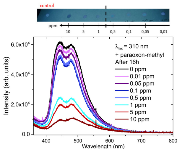
Fig. 8 NU-1000 emission intensity on cotton paper at different paraoxon-methyl concentrations (top) and measurements after 16 h using a portable spectrometer at \lambda_{\text{ex}} = 310 nm (bottom).
