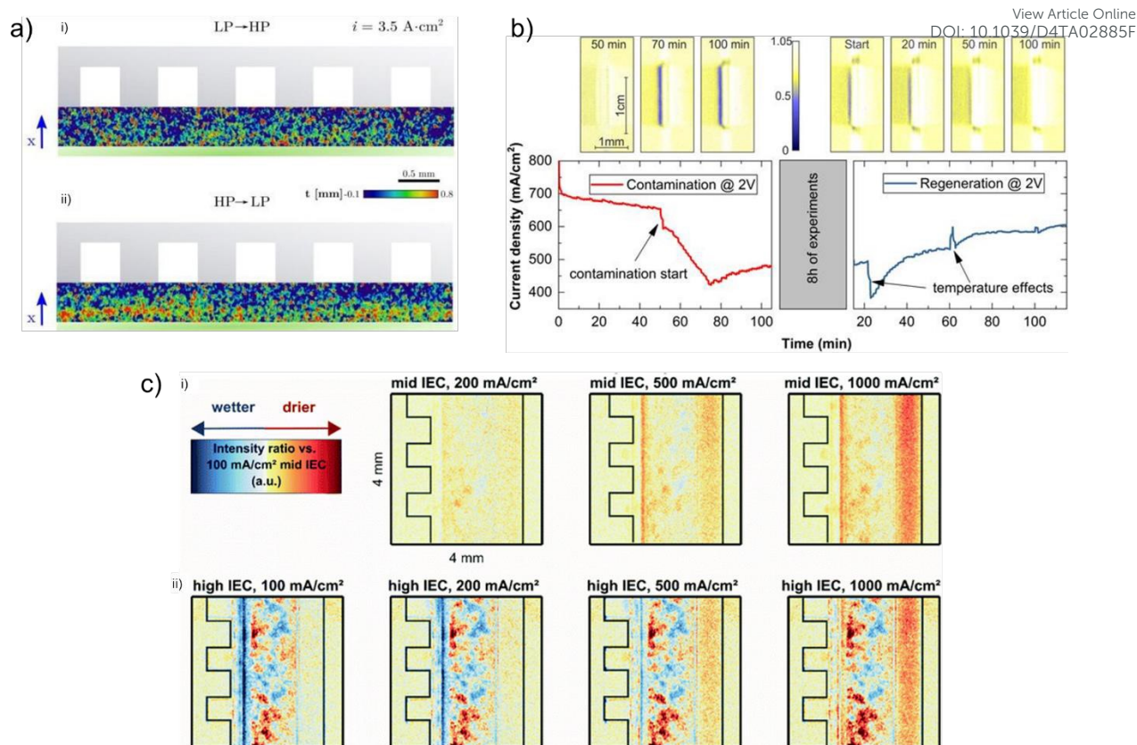
Figure 9 a) i) distribution of water and gas species in the low-to-high porosity (top) and ii) high-to-low porosity (bottom) region, where gas distribution is more homogeneous in the low-to-high structure as shown by the more uniform gas thickness (where blue-red colour indicates gas thickness from 0.1 – 0.8 mm). Reprinted from Lee et al. , 96 Copyright 2020, with permission from Elsevier. b) Diagram showing the diffusion of the \text{Gd}^{3+} gadolinium ions into the CCM with increasing duration, as indicated by the increasing amount of blue voxels with increasing time, and attempts to recover performance after 8 h of experiments, with the associated loss of \text{Gd}^{3+} as shown by the reduction in 'blue' voxels representing gadolinium ions. Reprinted under the terms of the Creative Commons Attribution 4.0 International (CC-BY 4.0) license, from Zlobinski et al. , 77 Copyright 2020, The Author(s), published on behalf of The Electrochemical Society by IOP Publishing Limited. c) Neutron radiographs showing the effect of ionomer additive on water accumulation at various current densities in an AEM electrolyser. The scale bar represents the change in neutron intensity in the PTL vs the 100 mA cm -2 mid IEC radiograph, where redder colours represent drier cases with less water, and bluer colours represent wetter cases with more water. Reprinted under the terms of the Creative Commons Attribution 3.0 Unported (CC-BY 3.0) license, from Koch et al. , 59 Copyright 2022, The Author(s), published by the Royal Society of Chemistry.
