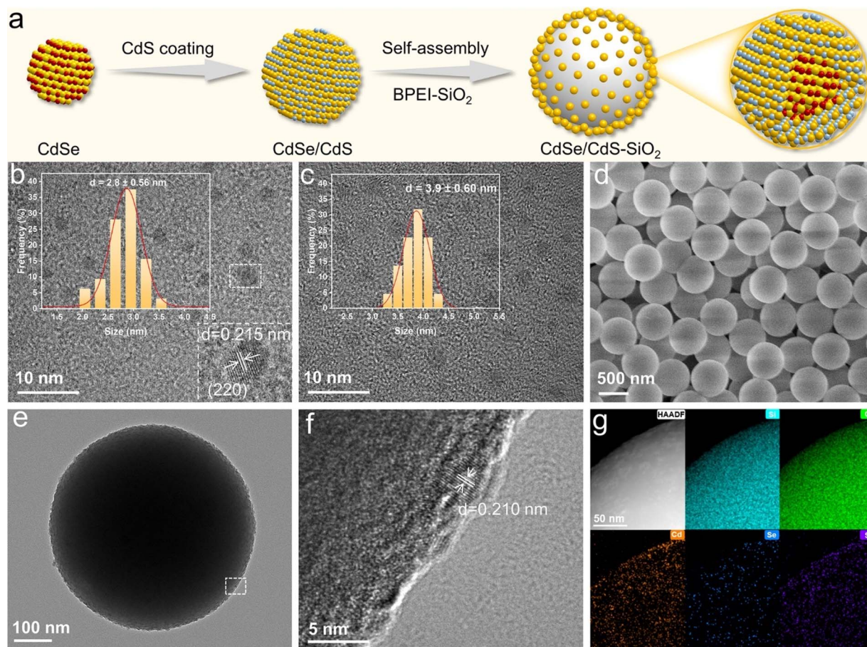
Fig. 1 (a) Schematic representation of the CdSe/CdS- \text{SiO}_2 composite synthesis procedure. HRTEM images of (b) CdSe QDs and (c) CdSe/CdS QDs (where 3 signifies approximately 3 atomic layers of the CdS shell). Inset: size distribution histograms of the corresponding QDs. (d) Scanning electron microscopy image of BPEI- \text{SiO}_2 spheres. (e) TEM image, (f) HRTEM image of the selected region in (e) and (g) high-angle annular dark field and corresponding elemental mapping images of the CdSe/CdS- \text{SiO}_2 composite.
