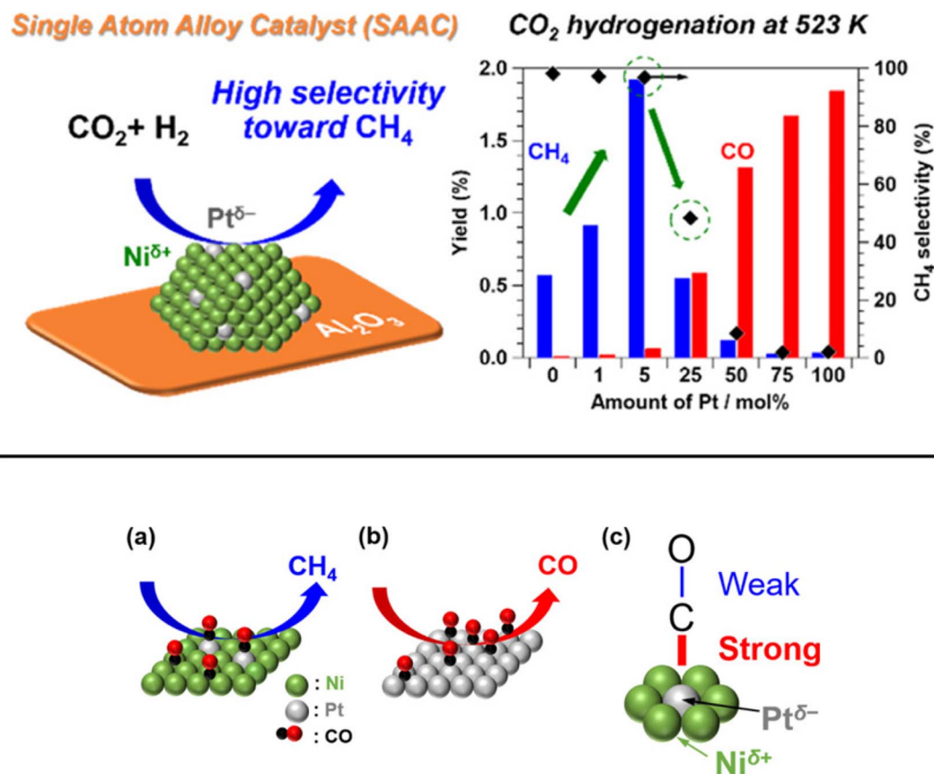
Fig. 13 Representation of the adsorbed \text{CO} species on the surfaces of the (a) iso-Pt catalyst and (b) bulk-Pt catalyst, and (c) the adsorbed \text{CO} model on a single \text{Pt}^{\delta-} atom encircled by \text{Ni}^{\delta+} atoms. Adapted with permission from ref. 141. Copyright 2019 American Chemical Society.
