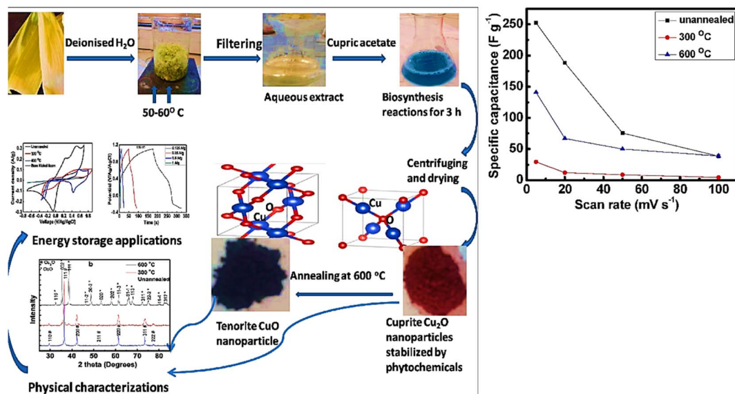
Fig. 7 Schematic of the procedure for the synthesis of \text{Cu}_2\text{O} NPs and their GCD response at different temperatures. 103
