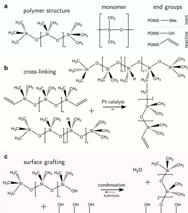
Fig. 2 Chemical structure of polydimethylsiloxane. (a) PDMS can be oligomeric ( n < 100 ) with low viscosity ( 1\text{--}5 \text{ mPa s} ) or assemble into long chains with high viscosities (up to \eta = 10 \text{ kPa s} ). The silicon–oxygen backbone provides chain flexibility while the methyl side chains yield water repellency. The end groups can be inert (trimethylsilyl) or reactive (hydroxyl, vinyl). (b) Hydrosilylation reaction between linear vinyl-terminated PDMS chains (top) and cross-linking agents with methylhydrosiloxane monomers create branches and networked elastomeric polymers. Here, the cross-linking agent is a polymer chain with x dimethylsiloxane and y methylhydrosiloxane monomers that are randomly arranged. The network branches are randomly distributed on the cross-linker chain and terminal on the PDMS base chain. (c) Hydroxyl-terminated PDMS chains can be grafted on surface hydroxyl groups that naturally occur on metals/metal-oxide, or can be functionalized with hydrogen plasma.
