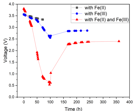
Fig. 3 Internal electrochemical discharge of Panasonic LIBs in individual 5 wt% potassium hexacyanoferrate(II) and 5 wt% potassium hexacyanoferrate(III) and in an electrolyte containing a 5 wt% solution of potassium hexacyanoferrate and potassium hexacyanoferrate.
