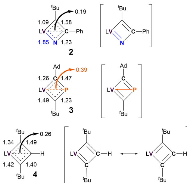
Fig. 6 Nalewajski-Mrozek bond orders of VCBF scaffolds and most probable resonance structures of 2–4. L = dBDI 2- = ArNC(CH 3 )CHC(CH 2 )NAr, Ar = 2,6- i Pr 2 C 6 H 3 .
