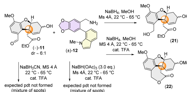
Scheme 5 Failed attempt towards reductive amination lactamization with galanthindolyl benzylamine.
