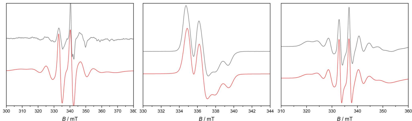
Fig. 6 X-band c. w. EPR spectrum of 1 mM 2Sc (left) in Et 2 O at 130 K, 2Y (middle) and 2La (right) in n Pr 2 O at 60 K. Black experimental, red simulations.
