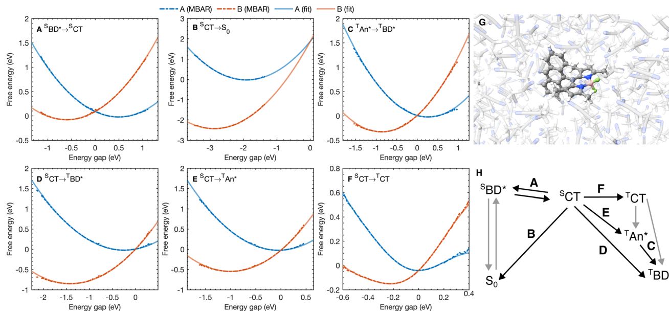
Fig. 3 (A–F) Free energy curves for the six A \rightarrow B processes considered with the reaction A \rightarrow B labeled on each figure. Points correspond to free energy curves calculated with MBAR and lines correspond to polynomials fitted to the MBAR cumulative distribution functions (see ESI† for details). (G) A snapshot for molecular dynamics simulations on the \text{S}_0 potential energy surface. (H) A scheme highlighting the processes in (A–F).
