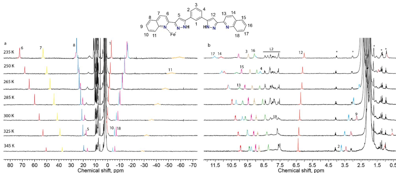
Fig. 4 Paramagnetic (a) and diamagnetic (b) regions of the ^1\text{H} NMR spectrum of (\text{Br}@\text{[Fe}(\text{L}2)_3]_2)^{3+} ( \text{CD}_3\text{CN} , 300 MHz) at various temperatures. The color coding designates the signals of the same proton at different temperatures to guide the eye. The signals corresponding to the free ligand are labelled as L2. Due to the low solubility of the complex in acetonitrile, the signals of small admixtures (such as grease, ethyl acetate and ^{13}\text{C} satellites of the residual solvent signals) appear magnified; they are designated by asterisks.
