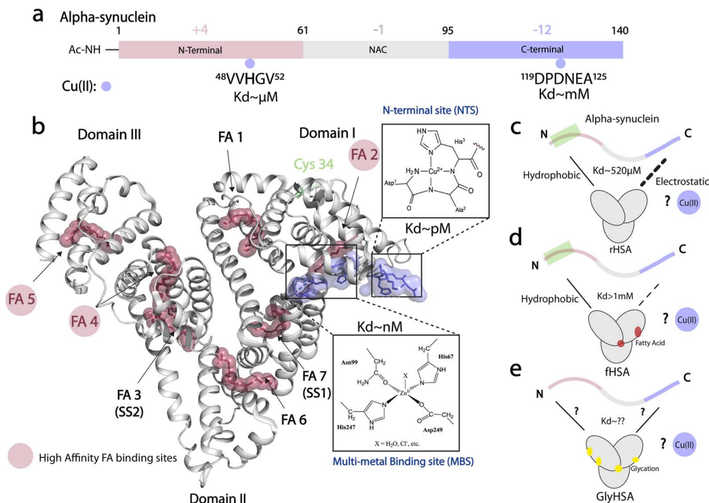
Fig. 1 \text{Cu(II)} binding properties of HSA, and monomeric alpha synuclein. (a) Monomeric alpha synuclein is comprised of three distinct regions: a positively charged N-terminal region spanning residues 1–60 (red), the non-amyloid- \beta component (NAC) region spanning residues 61–95 (grey), and the negatively charged C-terminal region spanning residues 96–140 (light purple). \text{Cu(II)} , represented by light purple spheres, binds N-terminal acetylated \alpha\text{Syn} (Ac- \alpha\text{Syn} ) at two different anchoring sites: the low affinity, non-specific metal binding site at the acidic DPDNEA segment, and the high affinity site at His-50. (b) Crystal structure of oleic acid bound HSA (PDB code: 1GNI). Oleic acid is shown as red spheres. High affinity fatty-acid binding sites are highlighted with a red circle (FA 2, FA 4 and FA 5), whereas low affinity sites are labelled in black. \text{Cu(II)} binding to HSA involves the ATCUN (amino terminal copper and nickel) binding site or N-terminal binding site (NTS). \text{Cu(II)} can also bind to the multi-metal binding site (MBS), but under physiological conditions, the MBS site is mostly occupied by \text{Zn(II)} . This structure was generated by merging the HSA crystal structure (PDB code: 1GNI) and the crystal structure of NTS model peptide DAKH complexed with \text{Cu(II)} ions (CCDC-809109) (c) HSA binds \alpha\text{Syn} monomers at the N- and C-termini through hydrophobic and electrostatic interactions, respectively. (d) The binding at the C-terminus is compromised upon FA binding to HSA. (e) The role that glycation of HSA plays in HSA- \alpha\text{Syn} interactions is unknown. (c–e) The role of \text{Cu(II)} ions in the \alpha\text{Syn} -HSA complex is also unknown.
