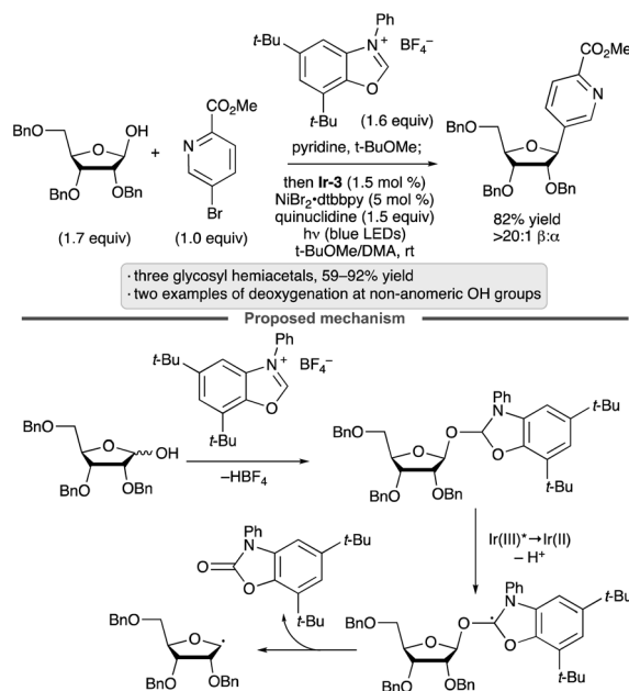
Scheme 19 Photocatalytic, deoxygenative arylations of alcohols mediated by an azolium salt. Ir-3 denotes [\text{Ir}(\text{ppy})_2(\text{dtbbpy})]\text{PF}_6 ; dtbbpy denotes 4,4'-di- tert -butyl-2,2'-bipyridine.
