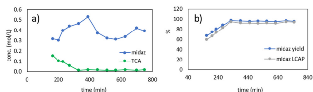
Fig. 14 Results of 13 hour production campaign. a) Molar concentration of TCA and midazolam in dissolution outlet b) instantaneous yield and LCAP of midazolam in dissolution outlet. LCAP = liquid chromatography area percent. Midaz = midazolam.
